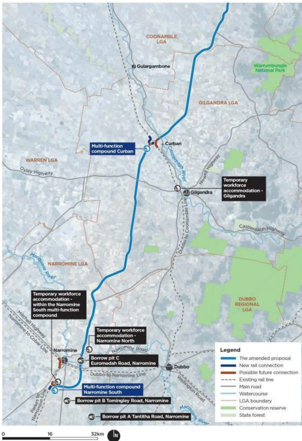
Figure 1 Narromine to Narrabri section of Inland Rail project footprint
