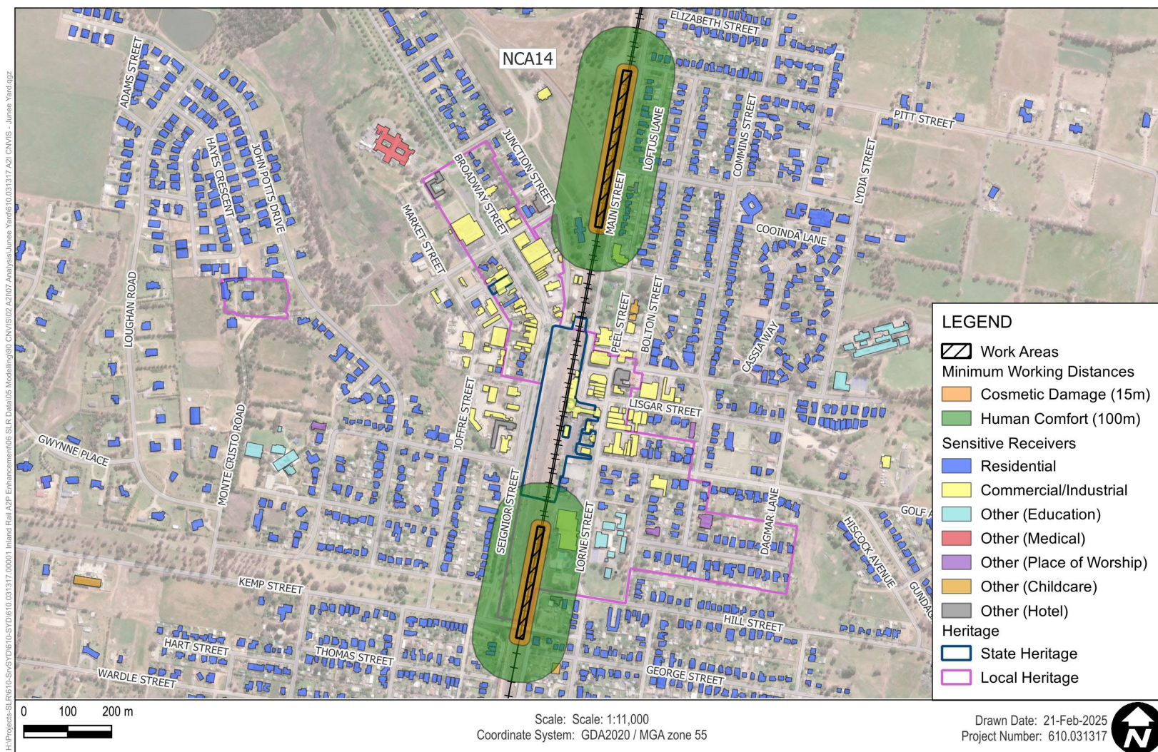
Figure 3 Construction Vibration Minimum Working Distances – Vibratory Roller <300 kN (7-13 tonne) (W.004)
