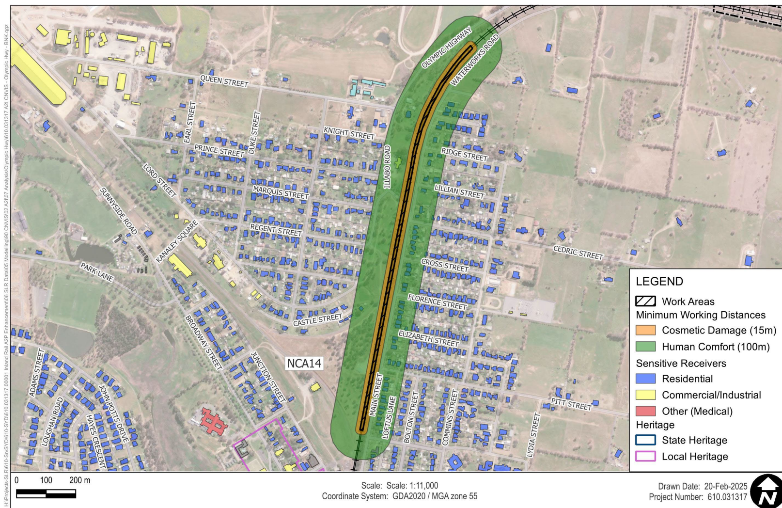
Figure 4 Construction Vibration Minimum Working Distances – Large Vibratory Roller <300 kN (7–13 tonne) (W.004)
