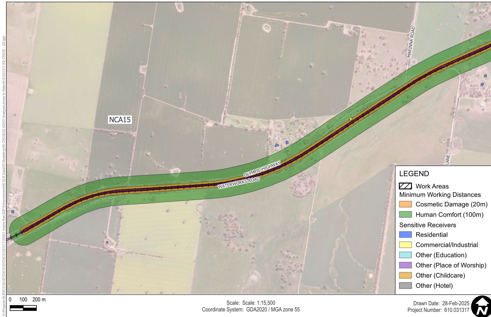
Figure 8 Vibratory Roller (13-18 tonne) - Minimum Working Distances W.005 (West)
