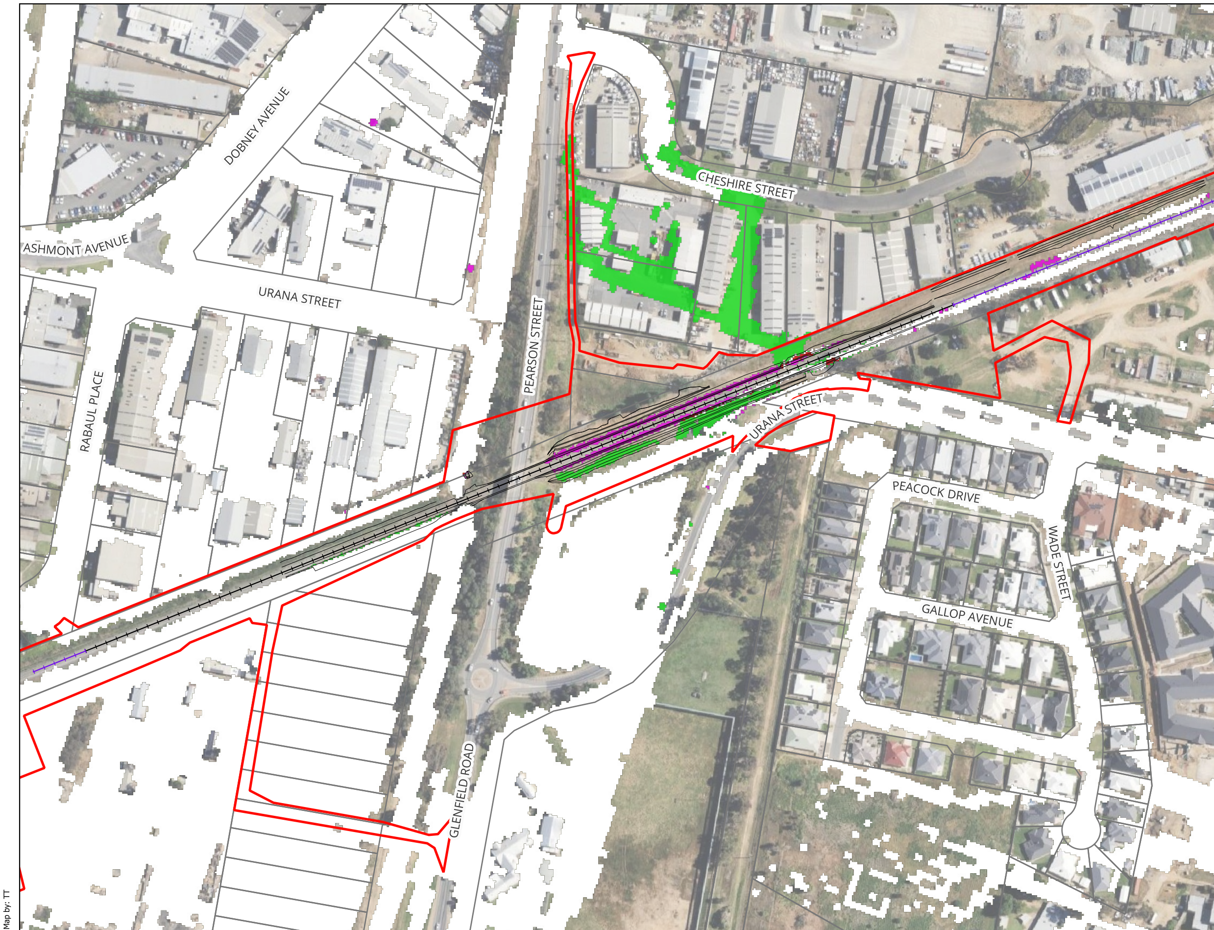
Figure A44 : Changes in Peak Flood Velocity for 2% AEP - Master Design Condition vs Existing Condition
