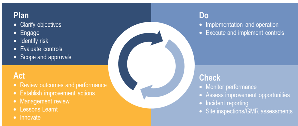
Figure 3-3 PDCA model
