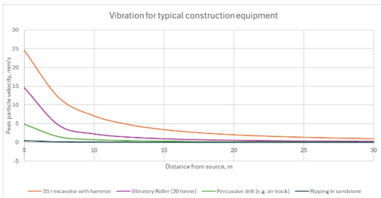
Figure 8-2 Vibration for typical equipment at various distances
