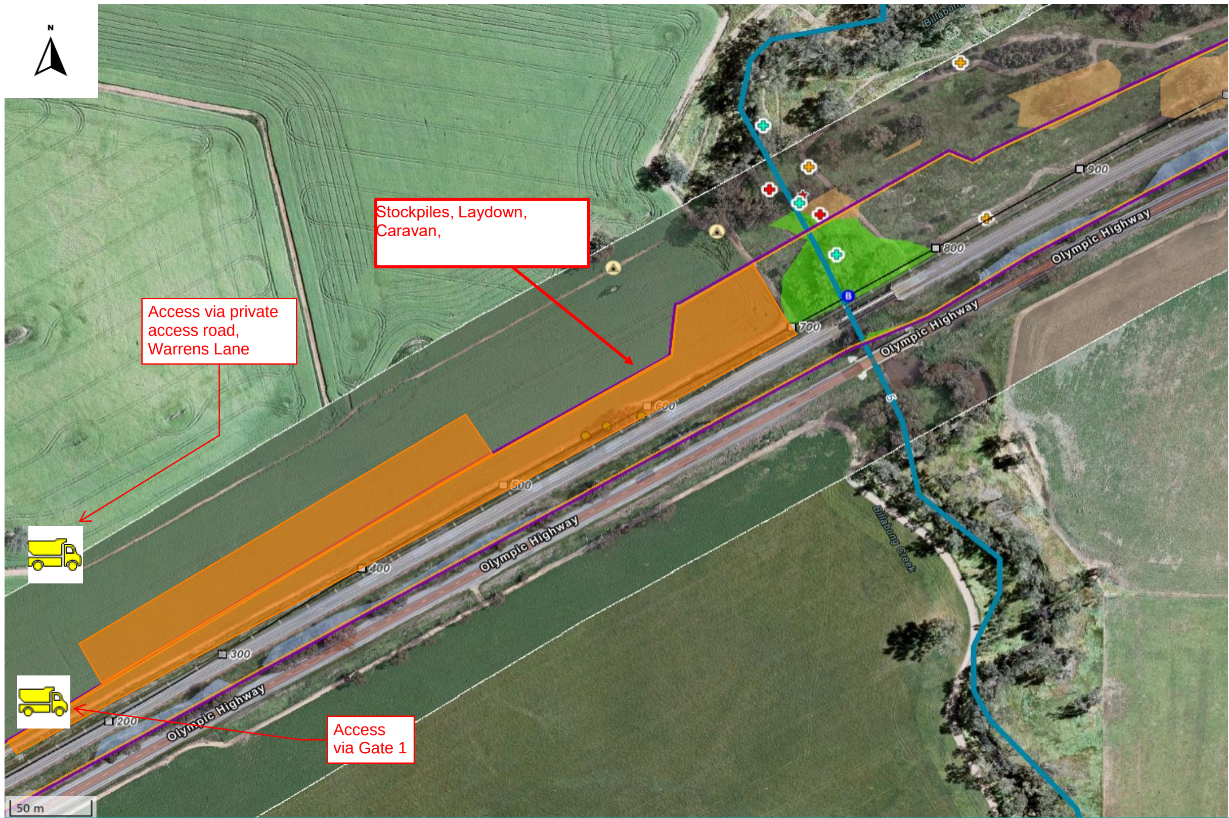
ILLABO TO STOCKINBINGAL Figure A8-1 Site Compounds
